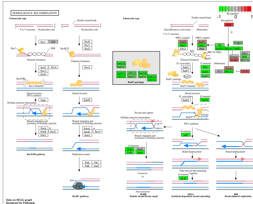
Figure 6: Homologous Recombination Pathway
