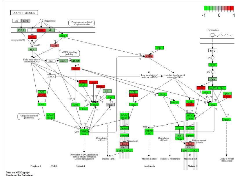
Figure 5: Oocyte Meiosis Pathway
