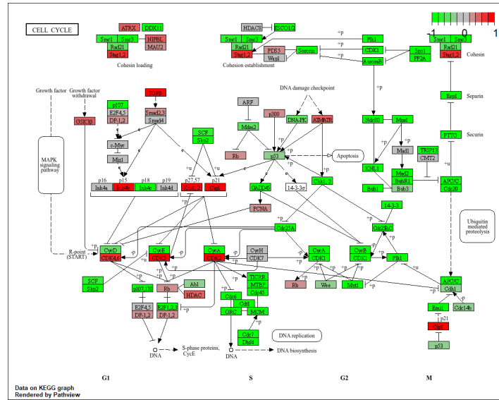
Figure 2: Cell Cycle Pathway
