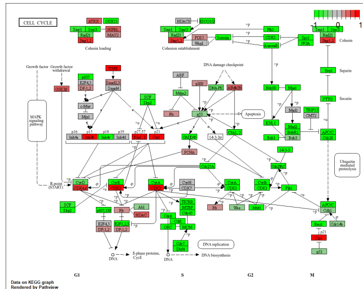
Figure 1: Cell Cycle Pathway Map
